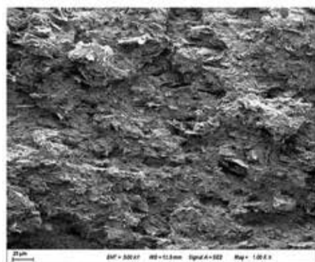
Fracture Surface from Tensile Tests PEEK + 15 wt% RGC39A
