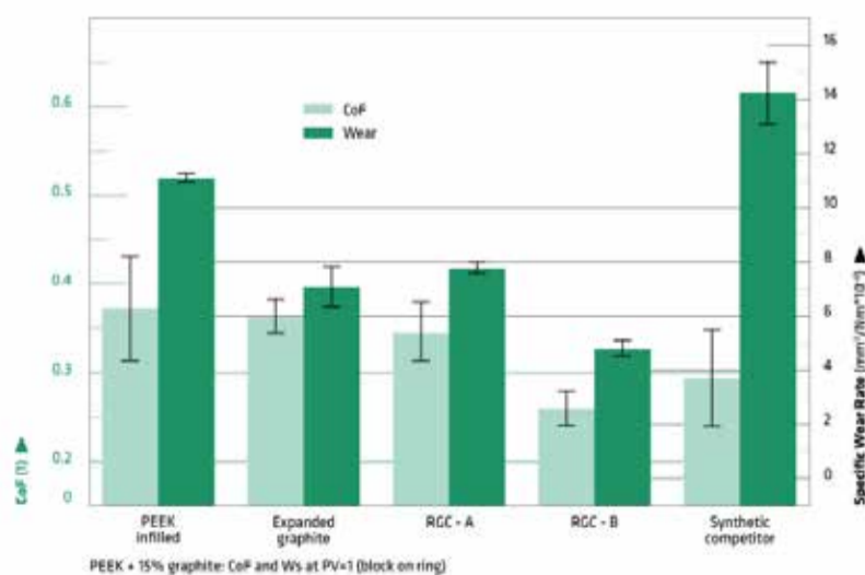
PEEK CoF and Wear Rate
